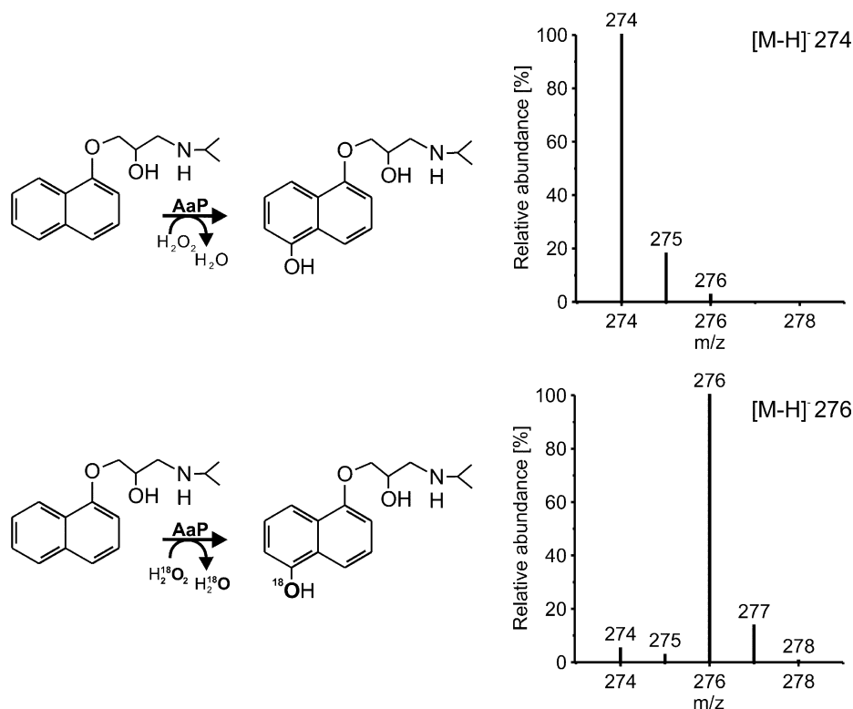
Figure 3. Mass spectra showing molecular ions of 5-OHP obtained from the oxidation of propranolol with AaP (1 U ml -1 , 0.2 μM) in the presence of natural abundance H 2 O 2 (top) or H 2 18 O 2 (bottom). 19
