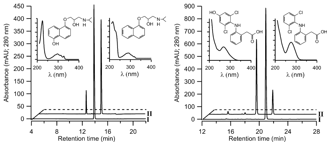
Figure 1. HPLC elution profiles showing products formed by AaP (2 U ml -1 , 0.4 μM) after conversion of propranolol (500 μM, left) and diclofenac (500 μM, right) in the presence of ascorbic acid (4 mM). Controls without enzyme (I). Complete reactions (II). The reactions (pH 7) were started by addition of H 2 O 2 (2 mM). Insets show UV/visible absorption spectra of the reactant (right) and major product (left) in each chromatogram. 18
